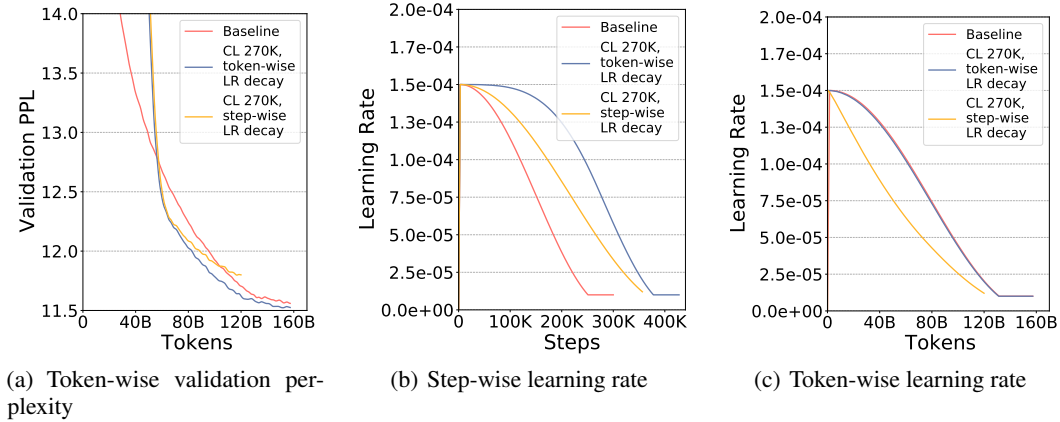
Figure 5: Validation perplexity and learning rate during GPT-2 1.5B SeqLen 1K pre-training with batch size 512, comparing the baseline and curriculum learning under different learning rate decay schedules (“CL 270K” means applying curriculum learning to the first 270K steps).
