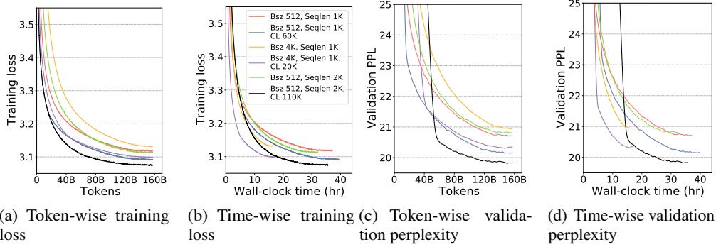
Figure 2: Training loss and validation perplexity during GPT-2 117M pre-training, comparing the baseline and curriculum learning under different batch sizes/LR and sequence lengths. All sub figures share the same legend as 2(b) (“CL 60K” means applying curriculum learning to the first 60K steps).
