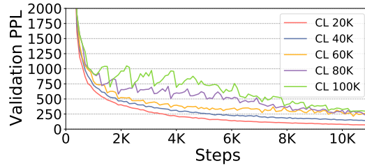
Figure 4: Step-wise validation perplexity during GPT-2 117M SeqLen 1K pre-training with batch size 512 and different curriculum learning duration. (“CL 20K” means applying curriculum learning to the first 20K steps).
